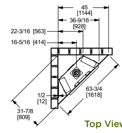
Top View Corner Installation
